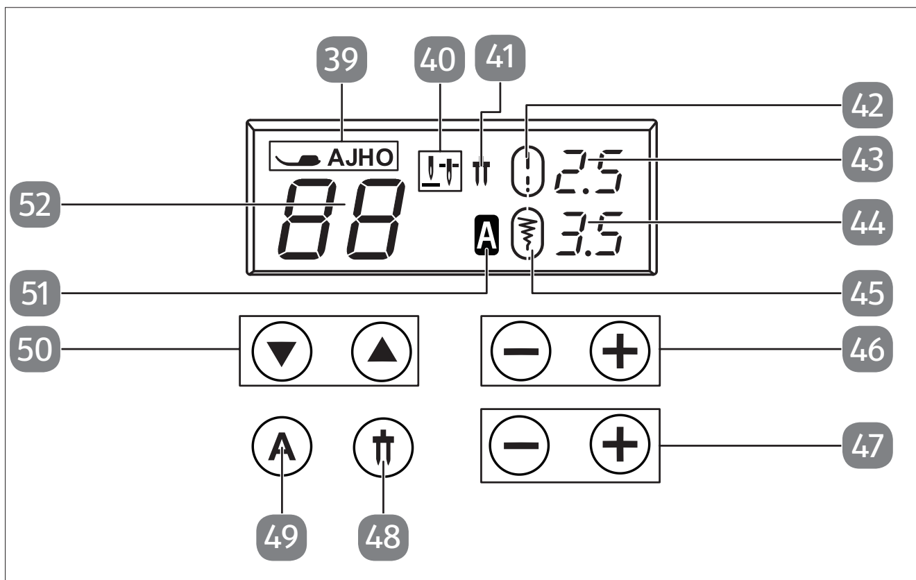
Fig. 4 – Display and control panel
